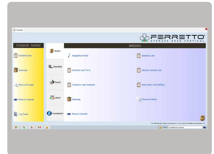
Home page
